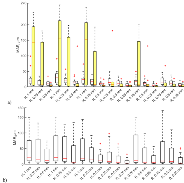
Figure 3.12. Box plots of MAE of estimated and theoretical motion signals evaluated in the middle scanning line starting from 11\ \text{mm} every 1\ \text{mm} to 29\ \text{mm} : a) radial motion detection, b) longitudinal motion detection. White and yellow boxes correspond to 1D cross-correlation and OpenOpticalFlow methods accordingly ( n=19 ). Median values are shown as a horizontal red line. Whiskers represent the minimum and maximum values. Outliers are indicated by red +. H – healthy volunteer, R – at-risk patient
