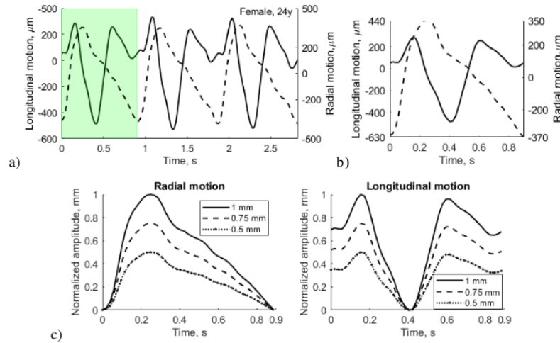
Figure 2.20. Motion signals post-processing for simulation of artery and tissue pulsation: a) in vivo radial (dashed line) and longitudinal (solid line) motion signals of CCA with preselected period (green shadowed area) which would be used to model artery and tissue pulsation, b) preselected heart cycle cut out from motion signals, c) motions signals amplitude normalization in three levels
