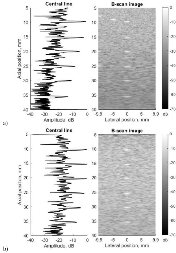
Figure 3.6. Comparison of scattering profile of point targets along central echoscopy line and whole B-scan images of a) measured US image of ATS Model 549 (physical wire phantom) b) simulated US image of digital wire phantom.
