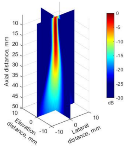
Figure 2.12. Simulation of linear array transducer pressure field in XZ and YZ planes. Element sub-divisions in the x-direction and y-direction were 1 and 9 accordingly
