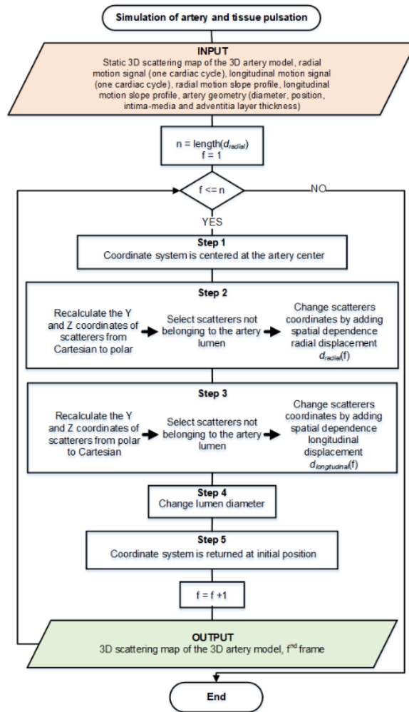
Figure 2.21. Functional diagram of Stage 2, simulation of the complex artery and tissue pulsation. Here f corresponds to the currently analyzing frame number in the motion signal and n – total number of such frames
