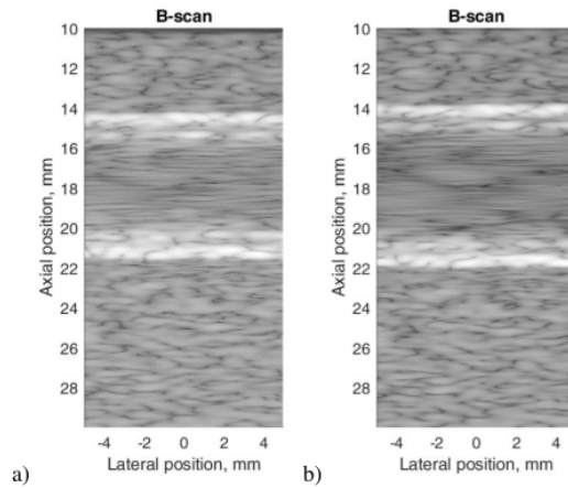
Figure 3.8. Simulated B-mode images of artery model at certain frames of the sequence: a) f_i and b) f_o . 23 years old male, motion amplitude were normalized to 1 mm
