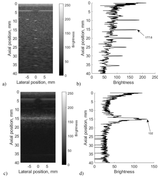
Figure 2.14. Determination of scatterers scattering strength in the digital phantoms: a) B-scan image of physical wire phantom, b) central echo line of B-scan image of physical wire phantom used for assignment of variance value for digital wire phantom, c) B-scan image of physical elevation plane phantom, and d) central echo line of B-scan image of physical elevation plane phantom used for assignment of variance value for digital elevation plane phantom
