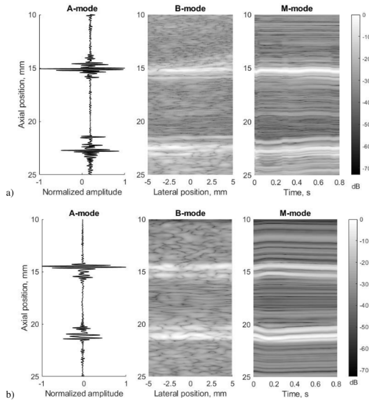
Figure 3.7. Comparison of RF signals form (A-mode, frame f_l , lateral position 0 mm), whole image (B-mode, frame f_l ), and movement over time (M-mode) according to the artery: a) in vivo (23 years old female, motion amplitude were not normalized) and b) in silico model data (23 years old female, motion amplitude were normalized to 1 mm)
