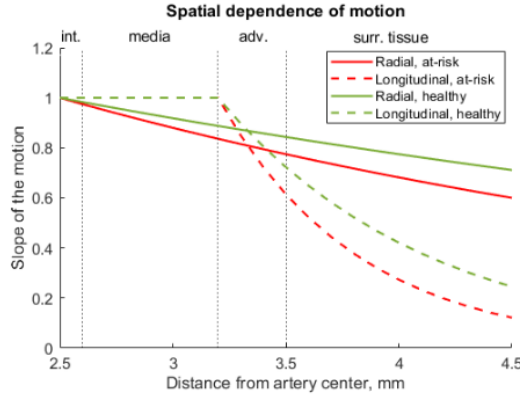
Figure 2.22. Spatial dependence of radial and longitudinal motions for healthy (slope of radial and longitudinal motions b_1=0.17 , b_2=1.08 ) and at-risk (slope of radial and longitudinal motions b_1=0.26 , b_2=1.62 ) subjects. The amplitude of radial motion is greatest at the surface of the artery (2.5 mm) and decreases exponentially into the surrounding tissues; the amplitude of longitudinal motion is greatest at the intima-media complex (at 2.5–3.2 mm), decreases significantly into the adventitia layer (3.2 – 3.5 mm), and finally, longitudinal motion amplitude is negligible in the surrounding tissues
