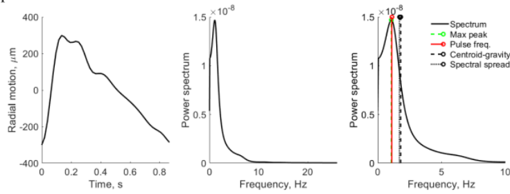
Figure 2.31. Averaged period of radial motion signal in the time domain ( left ), averaged period of radial motion signal in the frequency domain ( middle ), and spectrum with calculated frequency domain parameters in the range of 0-10 Hz ( right ). 53 years old female
