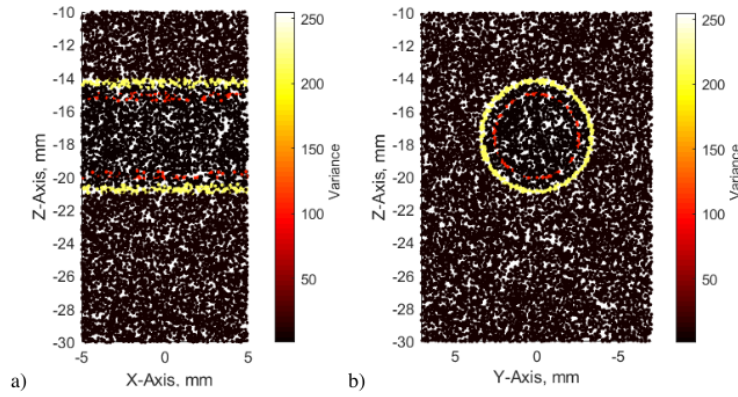
Figure 2.19. 3D map of scatterers at different viewpoints representing the artery model: a) longitudinal, b) axial
