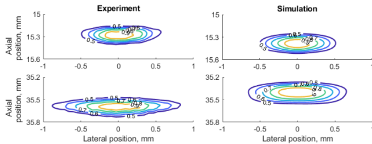
Figure 3.3. Comparison of PSF using isoline diagrams of RF signals reflected from targets at approximately 15 and 35 mm: experimental echoscopy of physical wire phantom (left column) and simulation of digital wire phantom (right column). Isolines presented at 0.1 intervals (from 0.5 to 0.9) of a normalized envelope of RF signals
