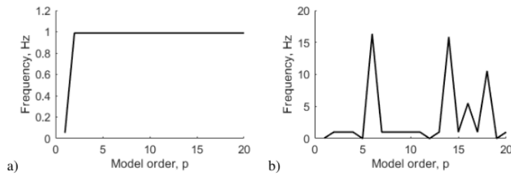
Figure 2.28. Frequency detection dependence on model order: a) Yule-Walker method and b) modified covariance method.
