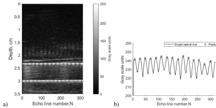
Figure 2.3. Evaluation of sampling resolution in lateral direction using the special phantom made using a fishing line: the B-scan image of the point targets (a) and single lateral line of the B-scan image with a seen point targets and preselected peaks whose position was used for evaluation of sampling resolution in the lateral direction (b)
