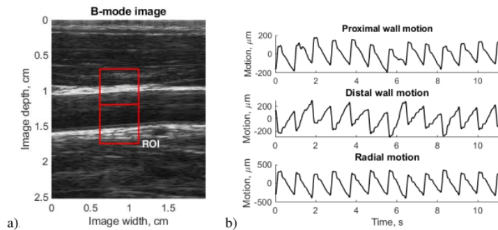
Figure 2.25. B-scan image with outlined ROI (a) and proximal, distal artery wall motion together with a total radial motion of CCA wall (b). The motion detected in the upper and lower part of outlined ROI corresponds to the proximal and distal wall motion accordingly. Summing the proximal and distal motion signals, the radial motion signals of the ROI were found. 53 years old female
