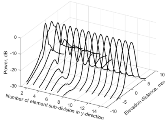
Figure 2.10. Representation of the main lobe and side lobe patterns at 15 mm axial distance from pressure field in YZ plane when a different number of sub-divisions in the y-direction of the element was used in the simulation
