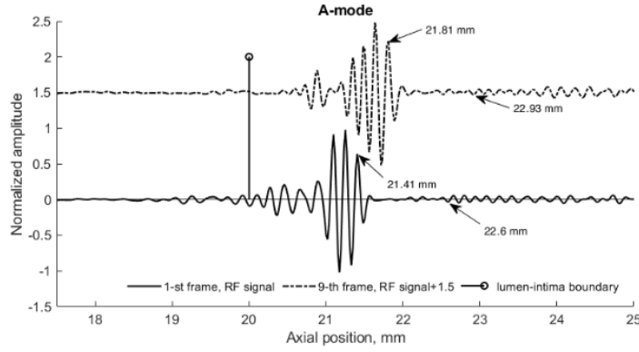
Figure 3.9. RF signals simulated by the model of a pulsating artery at frames f_1 and f_9 . Distal wall and surrounding tissues scattered RF signals (the artery center at 17.5 mm) depicting the radial wall displacement and its decrease in surrounding tissues. 23 years old male, motion amplitude was normalized to 1 mm
