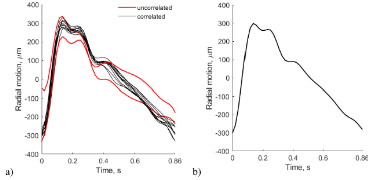
Figure 2.27. Detection of the average period for radial motion parametrization in time and frequency domain: a) periods of motion signal alignment according to the end of diastole and detection of both correlated and uncorrelated periods, and b) the average period of radial motion signal. 53 years old female
