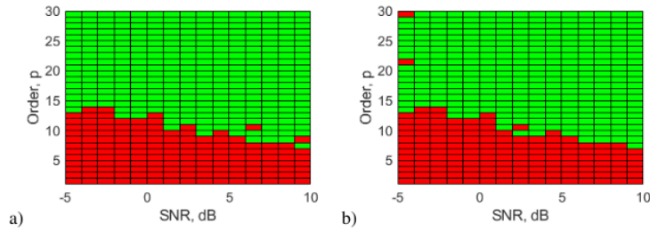
Figure 2.29. Frequency detection dependence on model order and SNR: a) Yule-Walker method and b) modified covariance method
