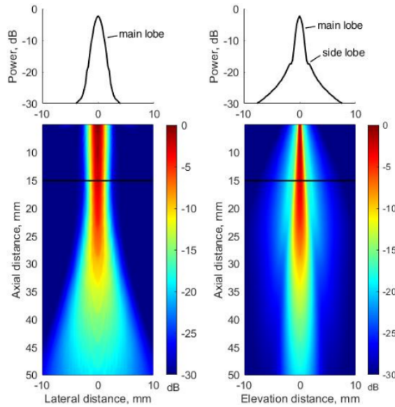
Figure 2.9. Simulation of linear array transducer pressure field in XZ plane ( left ) and YZ plane ( right ). Black lines at a 15 mm axial distance depict the position from where the main lobe and side lobe patterns are taken and represented above the corresponding pressure field. Sub-divisions in the x-direction and y-direction were the same and equal to 1
