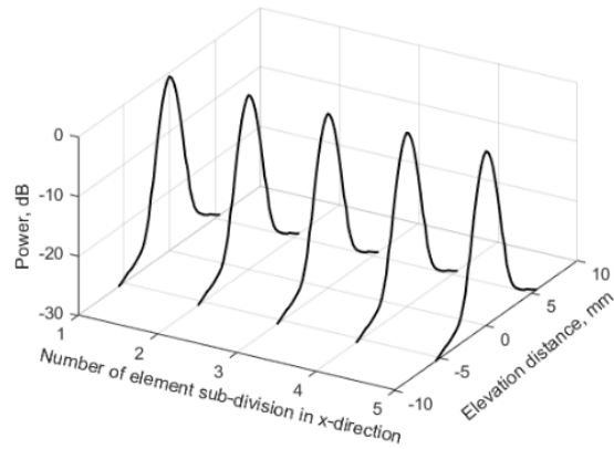
Figure 2.11. Representation of the main lobe and side lobe patterns at 15 mm axial distance from pressure field in XZ plane when a different number of element sub-divisions in the x-direction was used in the simulation
