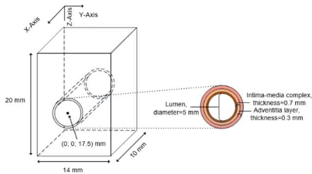
Figure 2.17. The general geometry of the artery model
