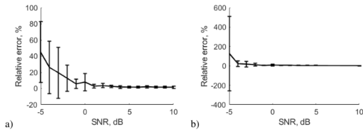
Figure 2.30. The relative error between modeled and detected frequency dependence on SNR: a) Yule-Walker method (model order const.=14) and b) modified covariance method (model order const.=14). Errorbar represents the mean and standard deviation of relative error (n=40)
