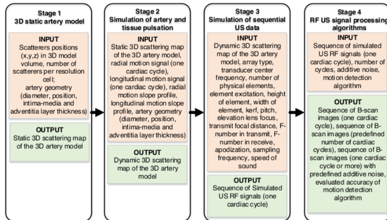
Figure 2.16. Overall simulation algorithm flow
